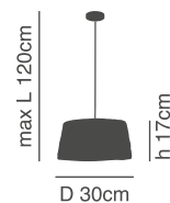
77-3637-37 L-G-1707 1xE27, max 60W, 230V
